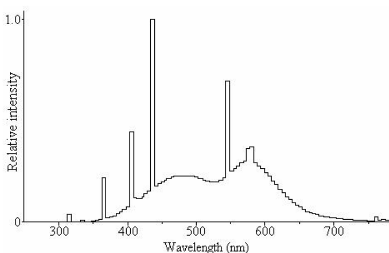
Fig. 1. Spectral characteristics of lamps emitting daylight by Philips (TLD 36W/54)
