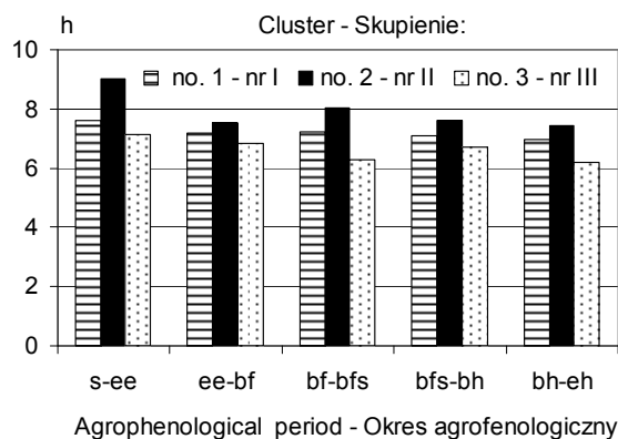
Fig. 5. Average values of sunshine duration in agrophenological periods of field cucumber calculated for each cluster
