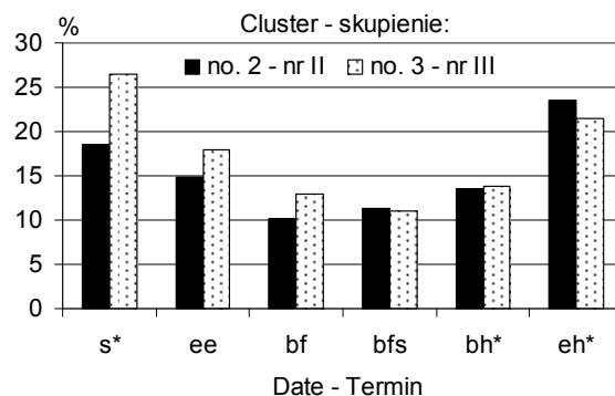
Fig. 4. Frequency of the occurrence of agrotechnical* and phenological dates of field cucumber for cluster 2 (below the determined average periods) and cluster 3 (above the determined average periods)
