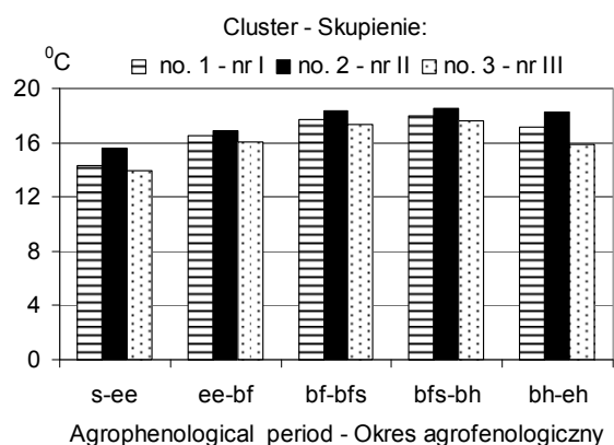
Fig. 6. Average air temperature values in agrophenological periods of field cucumber calculated for each cluster
